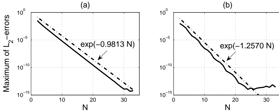
Figure 8: The maximum L_2 -error on 0.5 \leq t \leq 2.5 , as defined by the quantity M_N in (5.9). In (a) the parabolic contour is used with parameter values (3.12), and in (b) the hyperbolic contour with parameter values given in Table 1. Solid curves represent actual errors and dash-dot lines their theoretical estimates.
