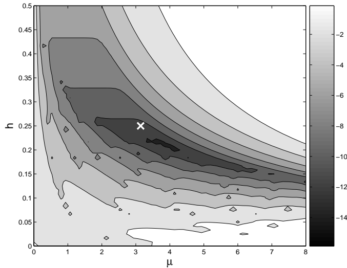
Figure 3: Contour plot of \log_{10} |f(t) - f_{h;N}(t)| , where the test problem is defined by (1.7), with \lambda = 0 , t = 1 . Here the parabolic contour is used, with N = 12 . The cross represents the parameter estimates (3.9).
