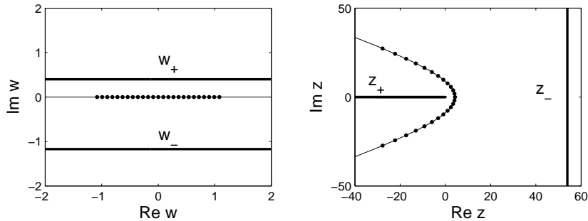
Figure 5: Same as Figure 2, but for the hyperbolic contour.
